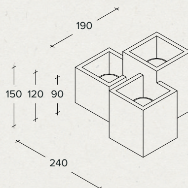
Three-lights plaster ceiling lamp
